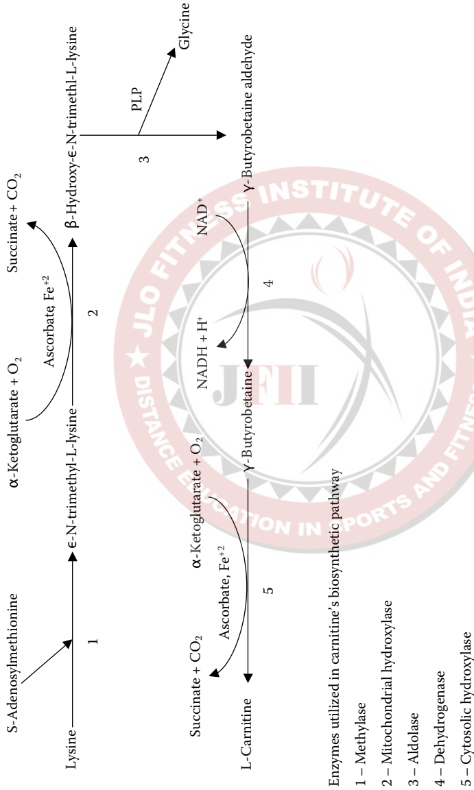
FIGURE 11.3 Carnitine biosynthesis.
